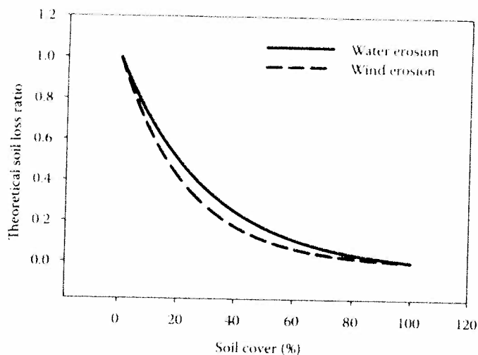
FIGURE 1.4 Soil loss ratios predicted by the revised universal soil loss equation (RUSLE) and revised wind erosion equation (RWEQ) with varying amounts of soil cover. Soil loss ratios include specified amount of residue cover for bare soil under high erodibility conditions. (Source: Merrill, S.D. et al. 2006. J. Soil Water Conserv. 61:7–13.)
