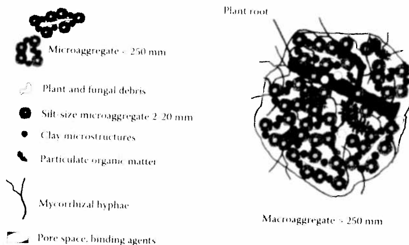
FIGURE 1.2 Soil macroaggregate formation. (Source: Jastrow and Miller, 1997. In Lal, R. et al., Eds., Soil Processes and the Carbon Cycle . CRC Press, Boca Raton, FL, pp. 207-223.)
