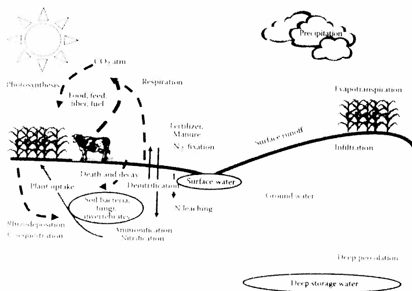
FIGURE 1.5 Interconnection of carbon, nitrogen, and water cycles.
