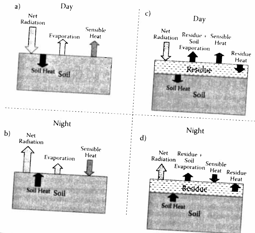
FIGURE 1.1 Energy fluxes for (a) bare soil during daytime, (b) bare soil during nighttime, (c) residue-covered soil during daytime, and (d) residue-covered soil during nighttime conditions. Arrows indicate directions of energy movement. Relative sizes of arrows approximate one potential scenario of dynamics of energy fluxes. Residue cover reduces energy gained (during daytime) and lost (at night) by dry soil surface. (Sources: Hillel, D. 1998. Environmental Soil Physics . Academic Press, San Diego, CA; Horton, R., K.L. Bristow, G.J. Kluitenberg, and T.J. Sauder. 1996. Theor. Appl. Clim. 54:27–37.)
