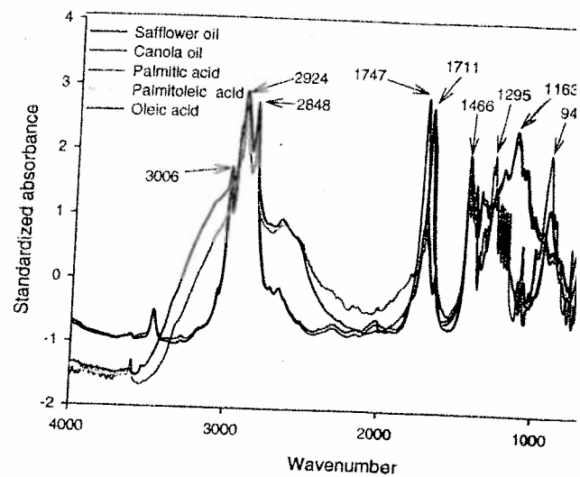
FIG. 2. Mid-infrared spectra of free fatty acids and oils.
