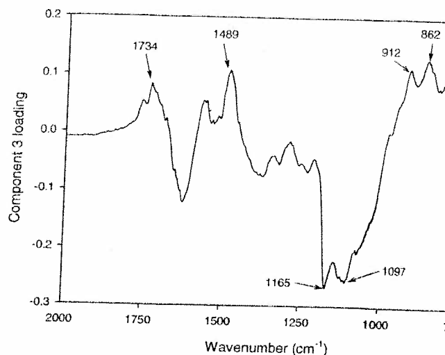
Fig. 9. Component 3 loadings for the PCA of the raw mid-infrared spectra of the mycorrhizal and non-mycorrhizal axenic cultures. The spectral range the highest loadings is shown.
