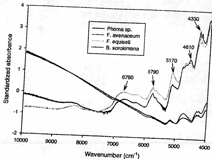
FIG. 5. Near-infrared spectra of fungal pure cultures.
