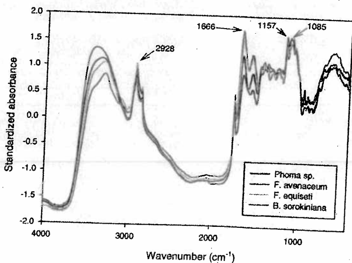
FIG. 4. Mid-infrared spectra of fungal pure cultures.
