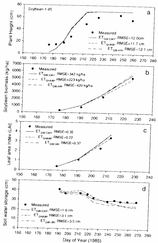
Fig. 5. Measured and ET_{SW-DAY} , ET_{SW-HR} , and ET_{SHAW} simulation results of (a) plant height, (b) aboveground biomass, (c) leaf area index (LAI), and (d) soil water storage for the Soybean-1-85 study.
