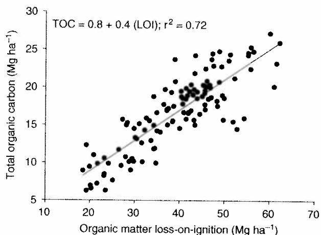
Figure 5. Relationship between two methods of measuring soil organic matter using soils from the 0–7.5 cm depth from contrasting management systems at eight locations in the Great Plains.
