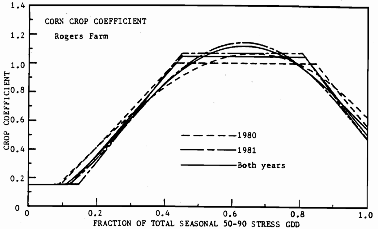
Figure 4. Overall corn crop coefficient values for the Rogers Farm for 1980 and 1981.
