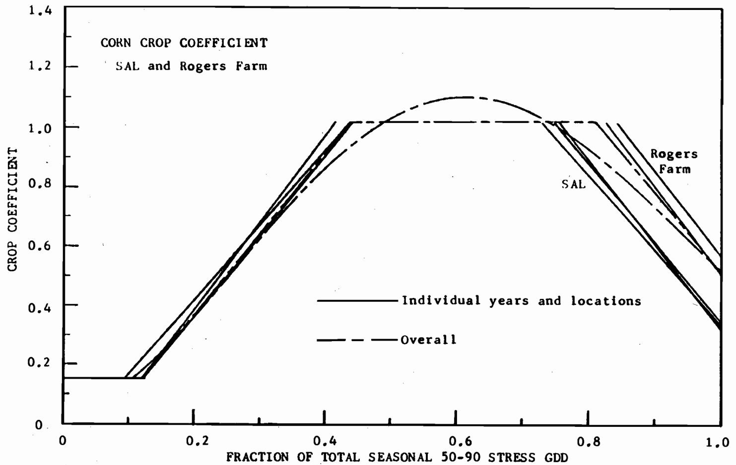
Figure 6. Overall corn crop coefficient values for the Rogers Farm and the Sandhills Ag. Lab.
