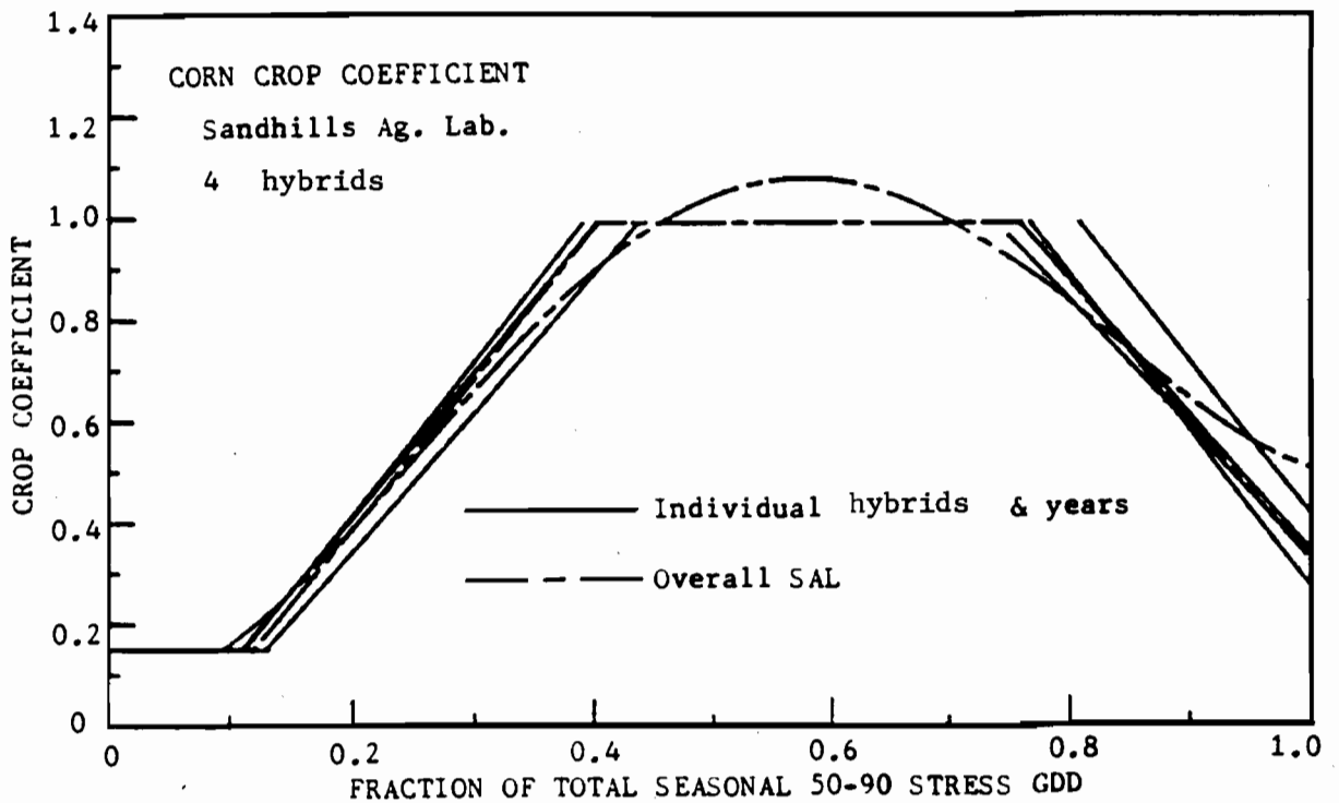
Figure 5. Overall corn crop coefficient values for the Sandhills Ag. Lab.
