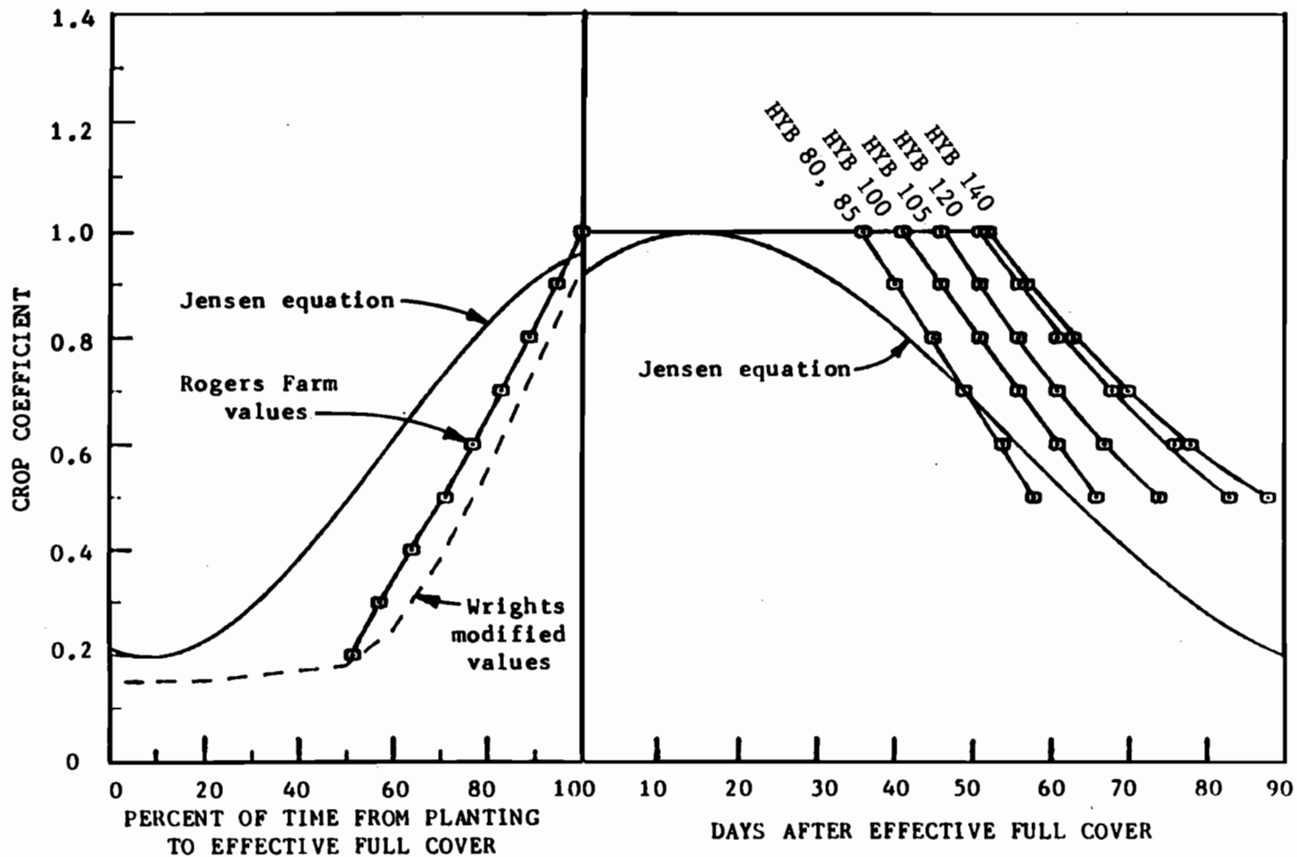
Figure 7. Comparison of the Rogers Farm crop coefficient results to Jensen's equations for corn and Wrights (1982) modified values.
