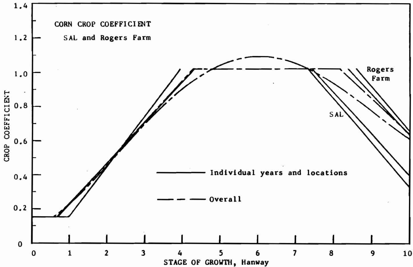
Figure 8. Overall corn crop coefficient values as a function of stage of growth for the Rogers Farm and the Sandhills Ag. Lab.
