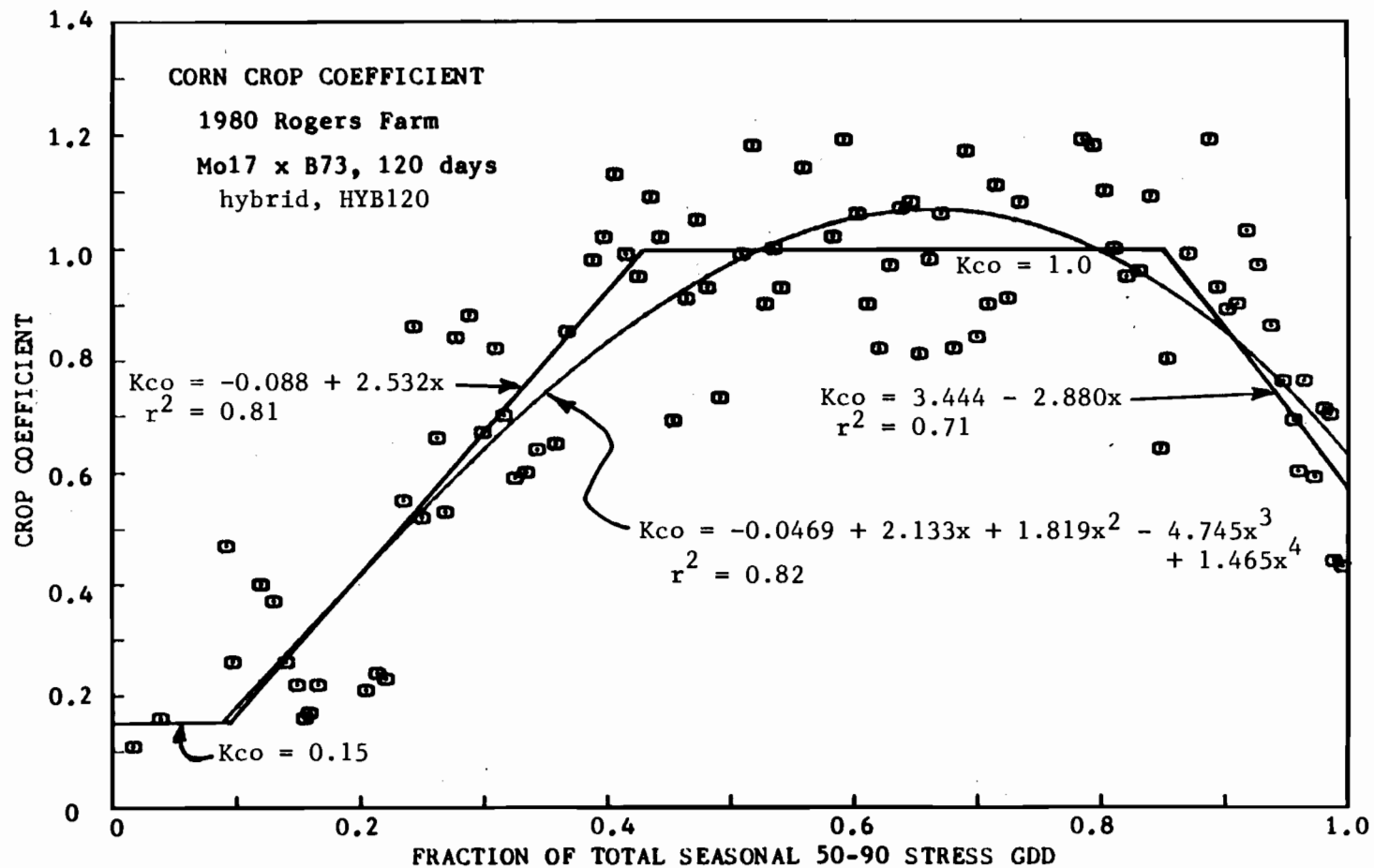
Figure 1. Corn crop coefficient results for HYB120 at the Rogers Farm during 1980.
