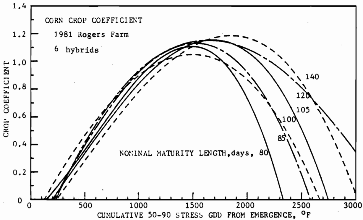
Figure 2. Corn crop coefficient values as a function of GDD for six hybrids at the Rogers Farm during 1981.
