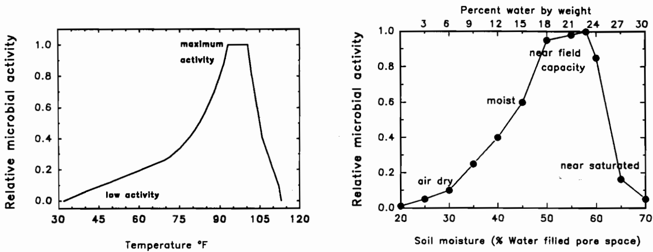
Fig. 1. Relative soil microbial activity as affected by soil temperature and soil moisture (water filled pore space).
