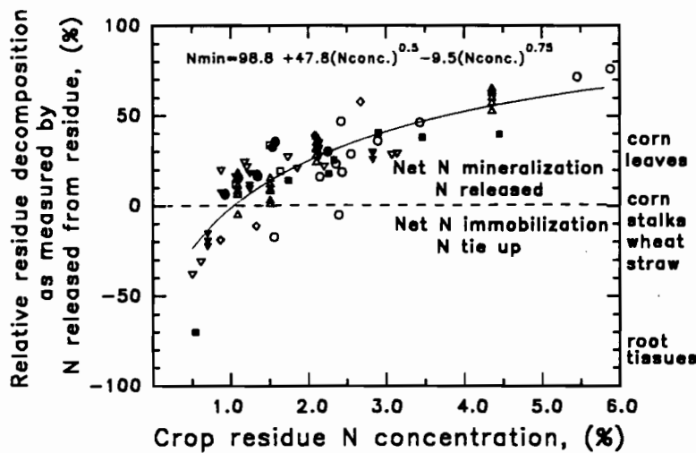
Fig. 2. Relative microbial decomposition of crop residues as affected by crop residue N concentration in the residue tissue as assayed by crop residue N release or tie up.
