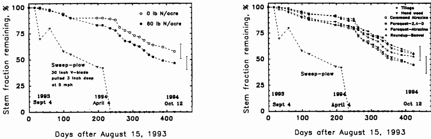
Fig 3. The percent of standing stems remaining in the field as affected by nitrogen and herbicide treatments over a 420 day period. Nitrogen applied broadcast as UAN (32 % N solution).
