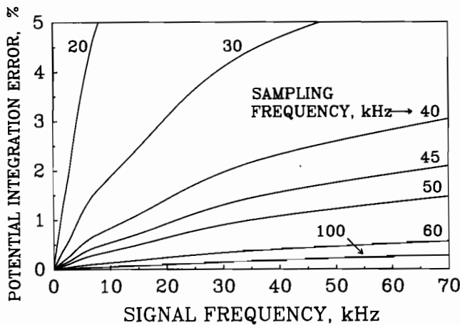
Fig. 4—Potential error of integrating water drop impact forces over time.
