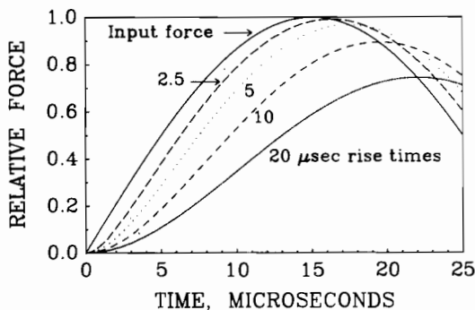
Fig. 2—Simulated sensor output responses to a sine-wave simulation of water drop impact forces.
