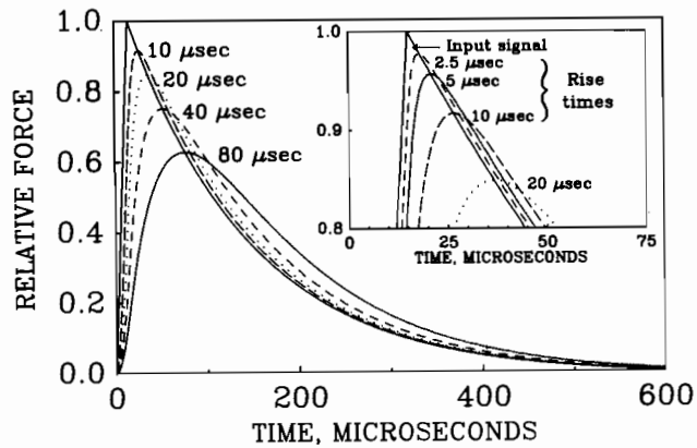
Fig. 1—Simulated sensor output responses to a linear-exponential simulation of water drop impact forces.
