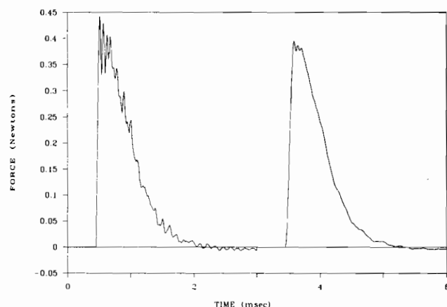
Fig. 5—An example recording of the forces of a water drop impacting the rough surface with the recorded signal on the left and the same signal smoothed on the right.
