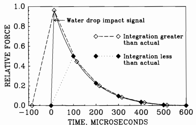
Fig. 3—Graphical example of potential integration error of water drop impact forces.
