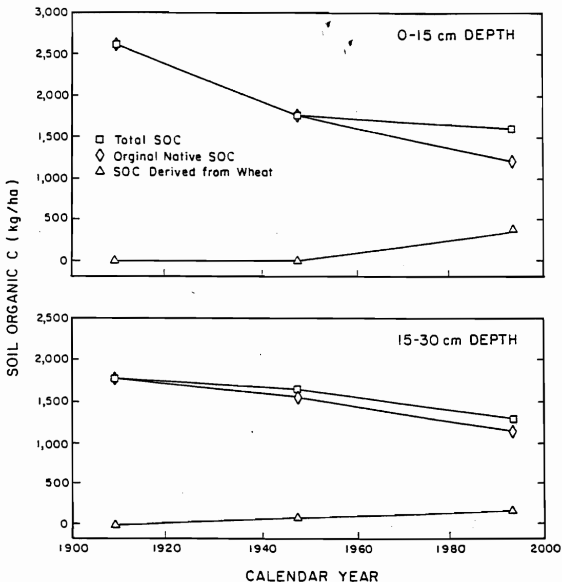
Fig. 2. Total soil organic C, original native soil organic C, and soil organic C derived from wheat from 1909 to 1993 at Akron, CO.
