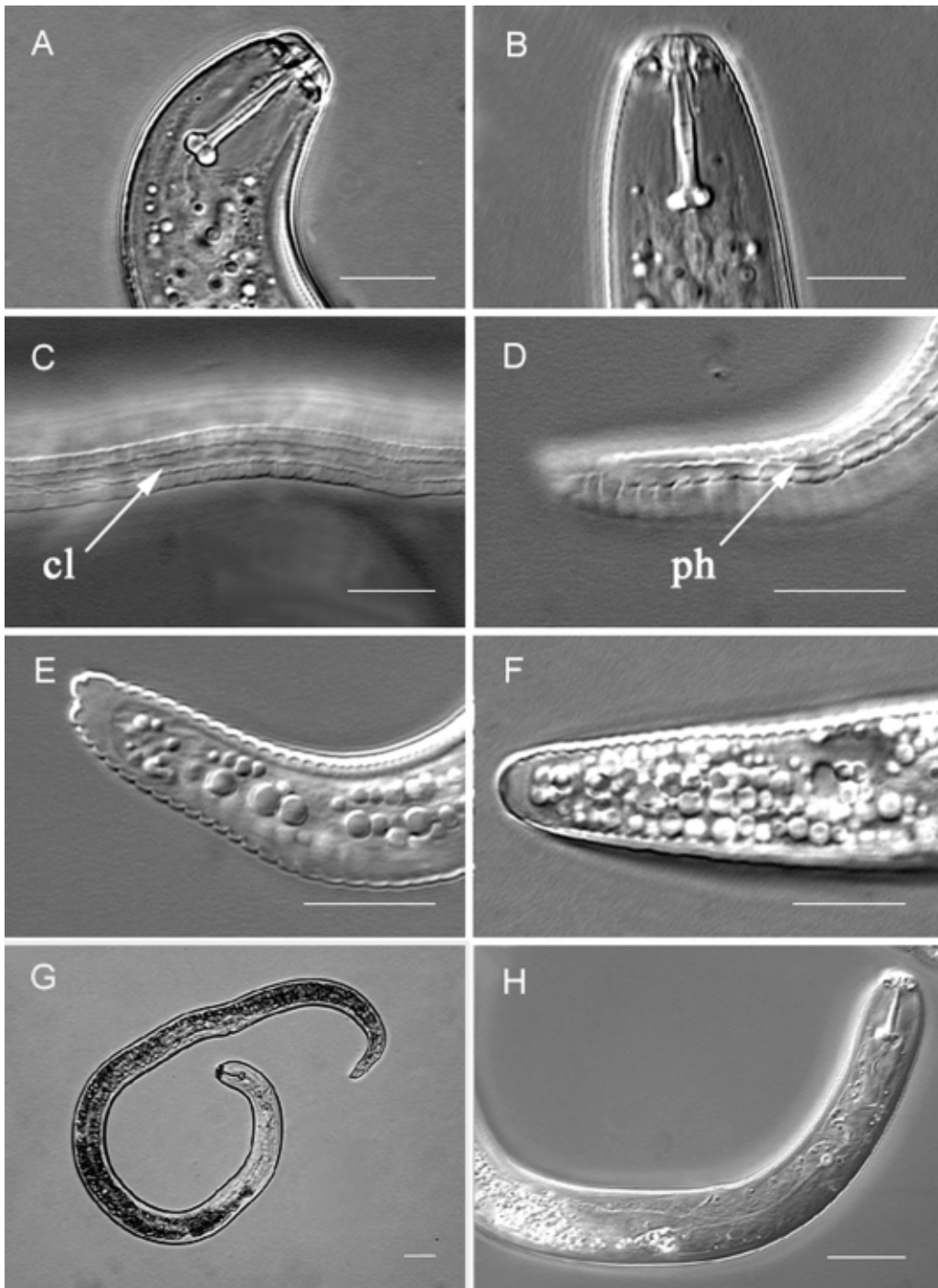
Fig. 2. Pratylenchus teres vandenbergae ; A: anterior end, stylet with rounded knobs and high lip region; B: anterior end, stylet with broadly rounded knobs; C: midbody lateral field with partial aerolation in outer rows and interrupted central line (cl); D: tail, lateral field and phasmid (ph); E: tail tip with asymmetrical projection; F: conoid tail tip with thickened cuticle; G: body, H: head and oesophagus. Scale bars: A–F = 10 \mu m, G–H = 20 \mu m.
