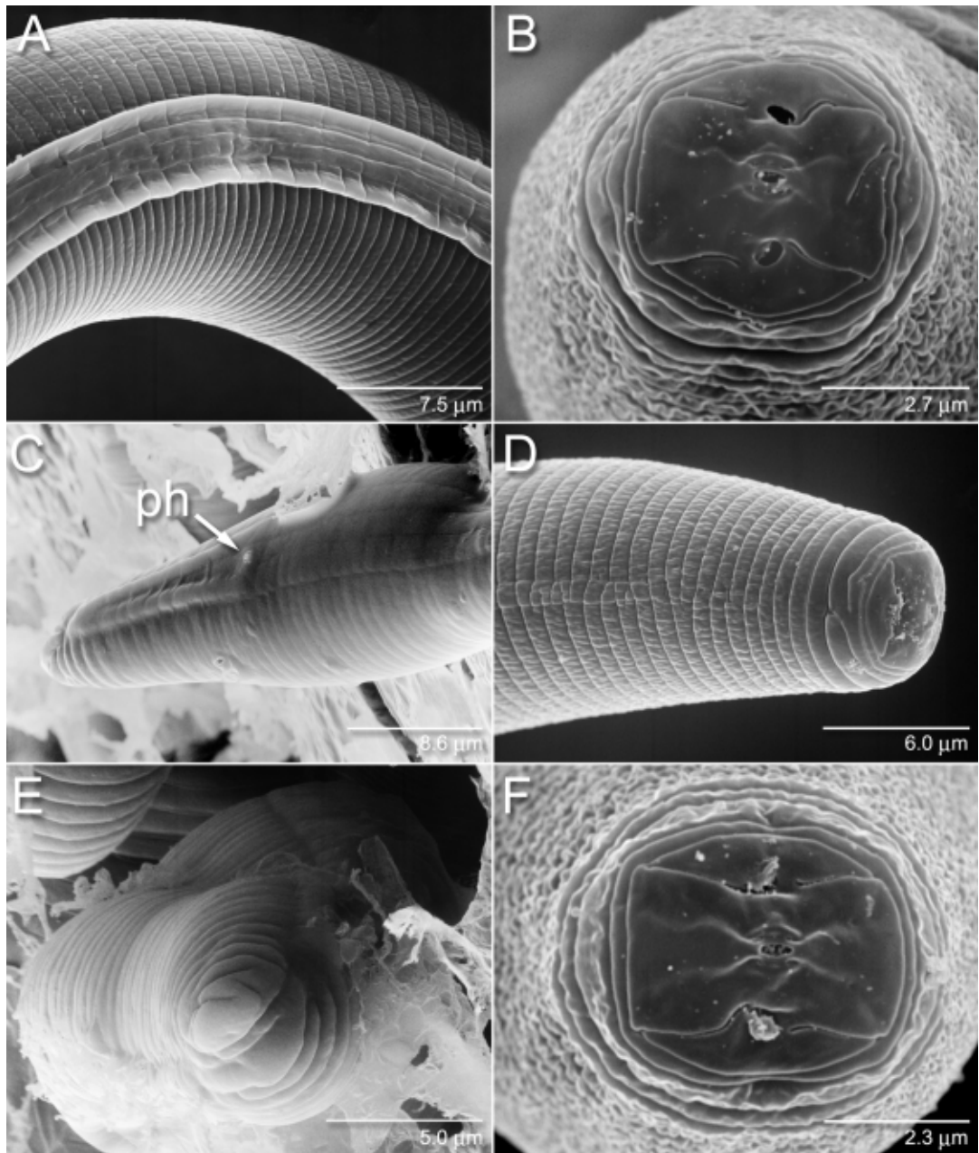
Fig. 3. Scanning electron micrographs. A: Pratylenchus teres vandenbergae , chemically-fixed lateral field; B: P. teres vandenbergae , chemically-fixed face view; C: P. teres JK, cryofixed tail with lateral field and phasmid (ph); D: P. teres vandenbergae , chemically-fixed anterior region with four lip annules; E: P. teres JK, cryofixed crenate tail tip; F: P. teres JK, chemically-fixed face view.
