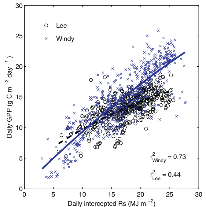
Fig. 7. Daily intercepted solar irradiance (Rs) plotted against daily gross primary productivity (GPP) for both fields. Lines show fitted curve for Windy (solid blue line) and Lee (dotted black line). Daily totals are summed from gap-filled half-hourly data. (For interpretation of the references to color in this figure legend, the reader is referred to the web version of this article.)
