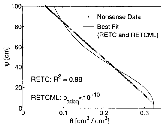
Fig. 2. “Fitting” S-shaped van Genuchten retention curve to synthetic data representing straight line. R^2 value is high even for this inadequate model, whereas p_{\text{adeq}} correctly reveals misfit.
