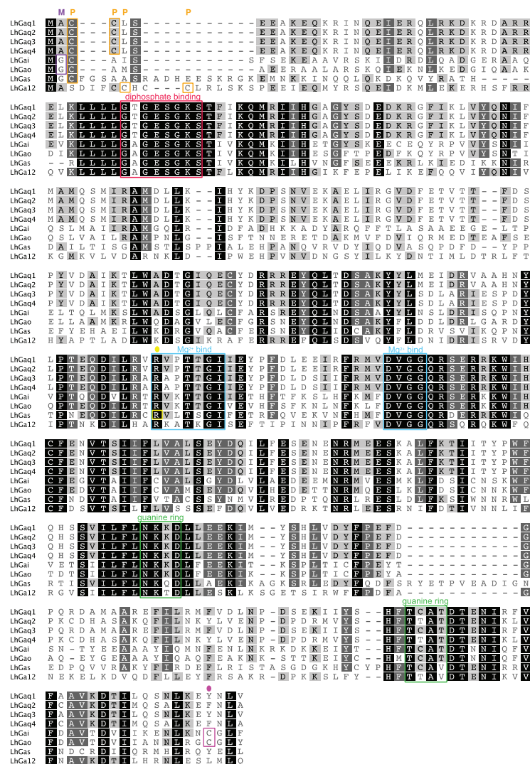
Figure 4. Multiple sequence alignment of L. hesperus Ga sequences. The respective full length L. hesperus Ga sequences were aligned in MUSCLE using default settings. Percent similarity shading is as in Figure 2. Conserved Ga subunit features/motifs are boxed: predicted myristoylation sites (purple M), predicted palmitoylation sites (orange P), diphosphate binding (red), Mg^{2+} binding (blue), guanine ring binding (green), putative cholera toxin-mediated ADP-ribosylation site (Arg186) in LhGas (yellow circle), putative pertussis toxin-mediated ADP-ribosylation sites (Cys352/Cys351) in LhGai and LhGao (pink circle).
