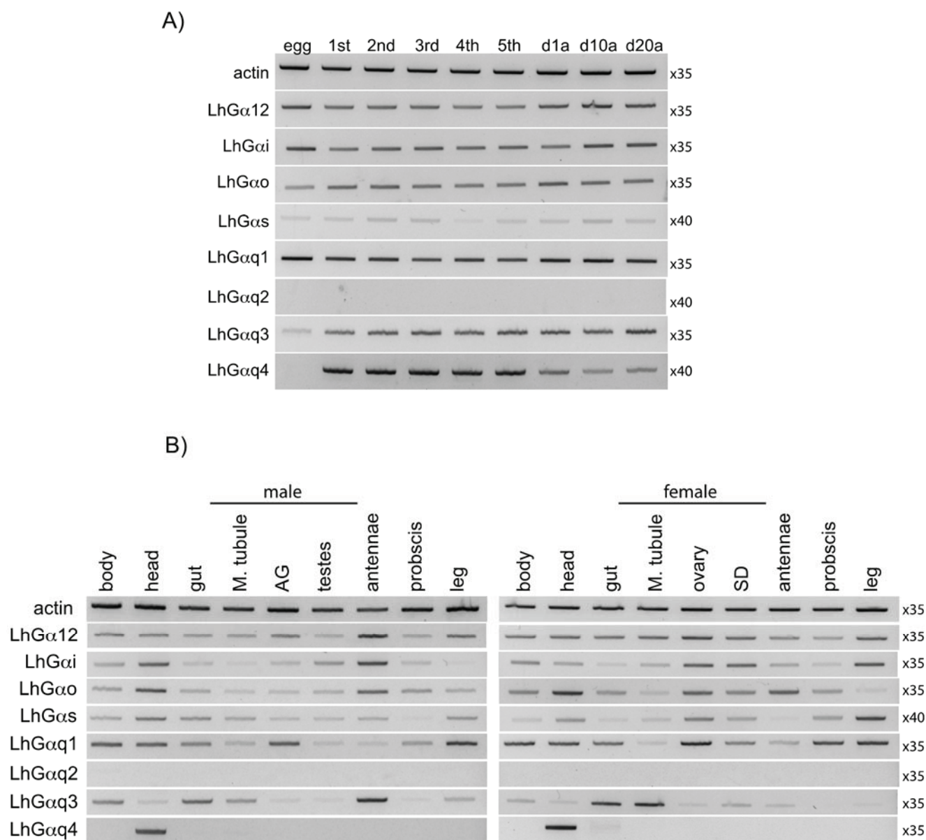
Figure 5. End point PCR-based expression profile of L. hesperus Ga transcripts. (A) Expression profile of LhGa sequences in eggs, nymphal development (1st–5th instars), 1-day-old mixed sex adults (d1a), 10-day-old mixed sex adults (d10a), and 20-day-old mixed sex adults (d20a); (B) Expression profile of LhGa sequences in sex-specific adult tissues. Abbreviations are: M. tubule, Malpighian tubule; AG, accessory glands (lateral and medial); SD, seminal depository. In both (A) and (B) , amplimers correspond to ~500–600 bp fragments of each transcript with products analyzed on 1.5% agarose gels stained with SYBR Safe. Negative images of the gels are shown for enhanced clarity of low expression transcripts. Numbers to the right of each gel image indicate the number of amplification cycles.
