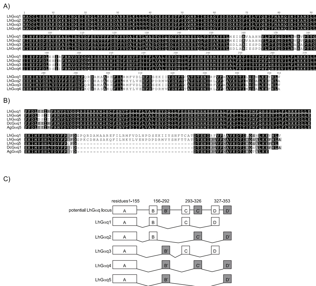
Figure 2. Alternative splice variants of LhGaα. (A) MUSCLE-based sequence alignment of LhGaα1-4; (B) MUSCLE-based sequence alignment of LhGaα5 with LhGaα1 and Gaα variants from A. gambiae (AAW50316; AgGaα5) and Diaphorina citri (XP_008479779; DcGaα1). The alignment corresponds to LhGaα1 amino acid residues 187–353. Shading denotes amino acid sequence similarity and is scaled as: 100% similarity (black), 99%–80% (dark grey), 79%–60% (light grey), and less than 59% (white); (C) Proposed alternative splice scheme utilized to generate the cloned LhGaα variants. Similar to A. gambiae and D. melanogaster , the LhGaα locus appears to have three homologous exons (B/B', C/C', and D/D') that are alternatively spliced to generate the five LhGaα variants. Putative exon-intron boundaries are based on observed sequence variations with coding sequences shown as boxes.
