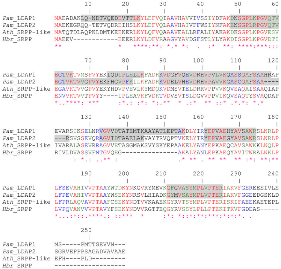
Figure 4. Polypeptide sequence alignment of avocado LDAP1 and LDAP2 ( Pam _LDAP1 and Pam _LDAP2) with the closest homolog from Arabidopsis ( Ath _SRPP-like; At3g05500) and the rubber tree SRPP ( Hbr _SRPP). Sequences were aligned using the ClustalW algorithm. Peptide regions of the two avocado proteins identified by MudPIT are highlighted in gray. Percentage coverage is 50% for LDAP1 and 41% for LDAP2.
