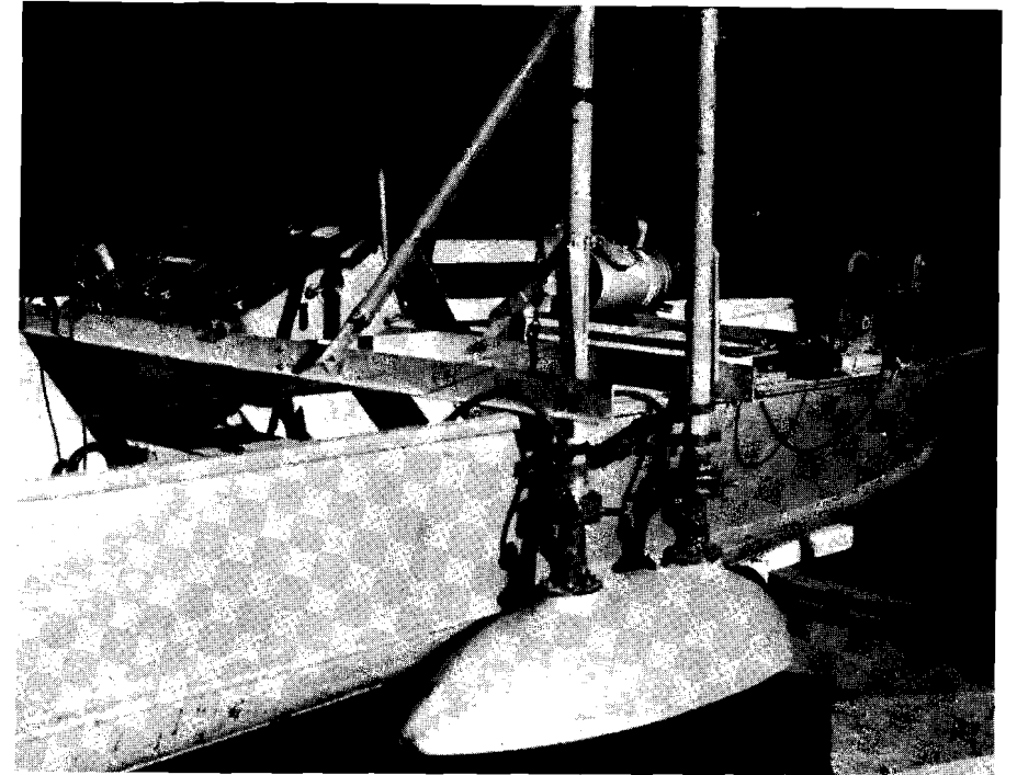
Figure 4. Mounting of fathometer transducer.
