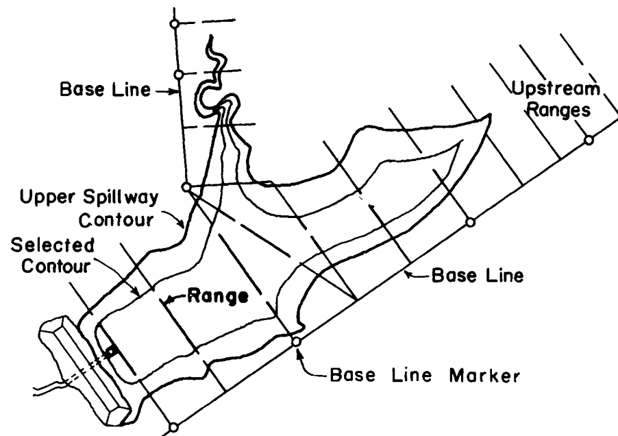
Figure 10. Suggested range layout for a typical reservoir.
