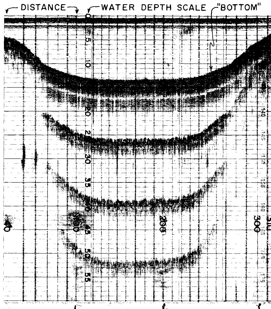
Figure 6. Fathometer chart showing distance and water depth.
