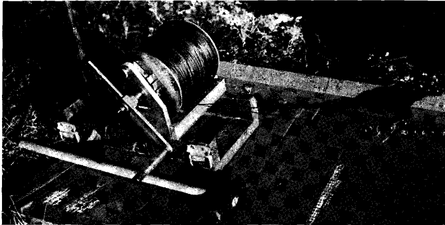
Figure 3. Reel holding cable which is stretched across reservoir to guide boat.
