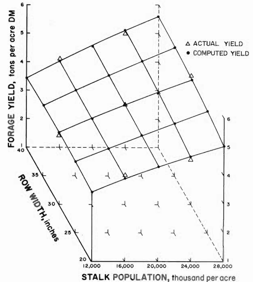
Fig. 10 Yield response (forage dry matter) surface from stalk population and row width. Pioneer 321 hybrid average for 1965 and 1966.
