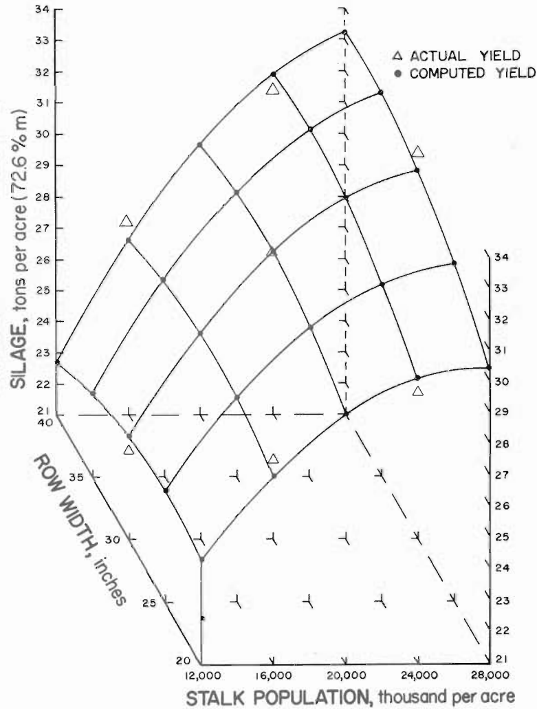
Fig. 8 Yield response (silage) surface from stalk population and row width. Pioneer 321 hybrid average for 1965 and 1966.
