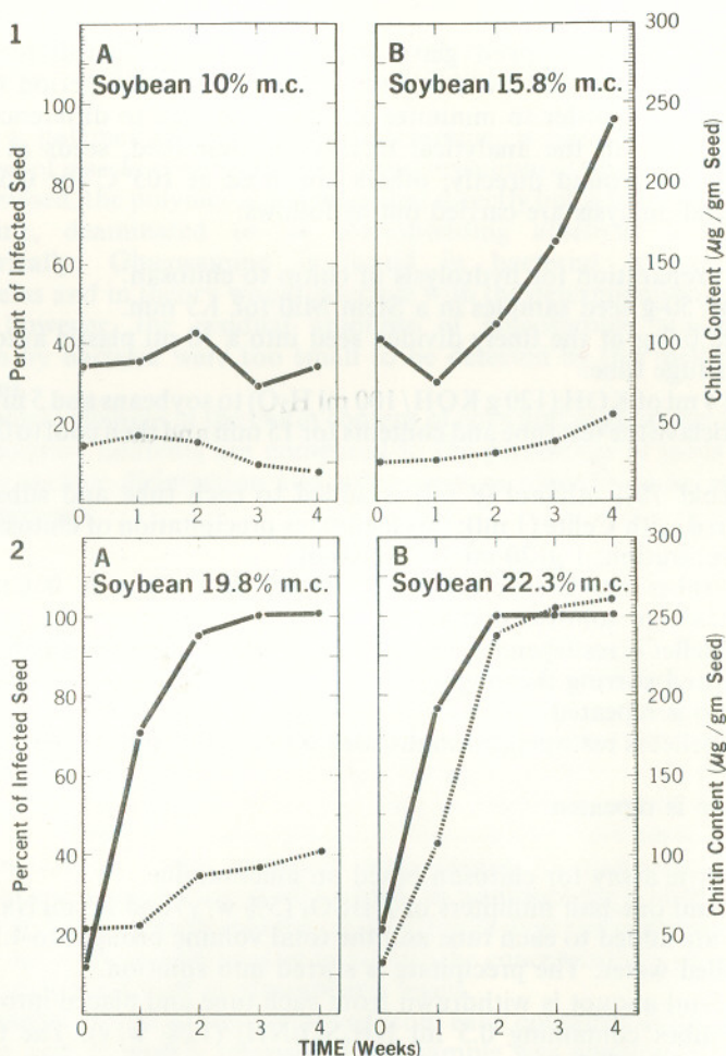
Fig. 1. Chitin content (broken line) and percentage of seed infected with fungi (solid line) of soybean seeds stored at various moisture contents for 1 month. The results are averages of duplicate samples. 1A: 10% moisture content; actual chitin values proceeding from 0 time to 4 weeks: 36.5^{\pm 6.4} , 42.6^{\pm 7.1} , 38.9^{\pm 7.3} , 24.0^{\pm 6.3} , and 19.5^{\pm 3.9} . Fungi isolated: Aspergillus glaucus , Alternaria sp. and Phoma sp. Percentage of seed that yielded fungi (PSYF) after surface disinfection at end of experiment was 33. 1B: 15.8% moisture content; actual chitin values are 24.7^{\pm 7.0} , 26.0^{\pm 6.4} , 29.4^{\pm 8.8} , 36.6^{\pm 3.6} , and 54.8^{\pm 6.2} . Fungi isolated Aspergillus glaucus (92-98%), Alternaria sp., Phoma sp. and Aspergillus candidus . PSYF = 92-98%. Fig. 2. Chitin content (broken line) and percentage of seed infected with fungi (solid line) of soybean seeds stored at various moisture contents for 1 month. The results are averages of duplicate samples. 2A: 19.8% moisture content: actual chitin values are 54.0^{\pm 8.6} , 56.8^{\pm 10.2} , 87.6^{\pm 18.9} , 92.1^{\pm 10.7} , and 102^{\pm 16.8} . Fungi isolated: Aspergillus glaucus (100%), A. candidus , Alternaria sp., Penicillium sp. and Phoma sp. PSYF = 100%. 2B: 22.3% moisture content; actual chitin values are 32.8^{\pm 4.6} , 107.8^{\pm 14.5} , 238.6^{\pm 36.0} , 254.8^{\pm 15.5} , and 261.5^{\pm 27} . Fungi isolated: Aspergillus glaucus (98%), A. candidus , Penicillium sp., Alternaria sp. and Phoma sp. PSYF = 100%.
