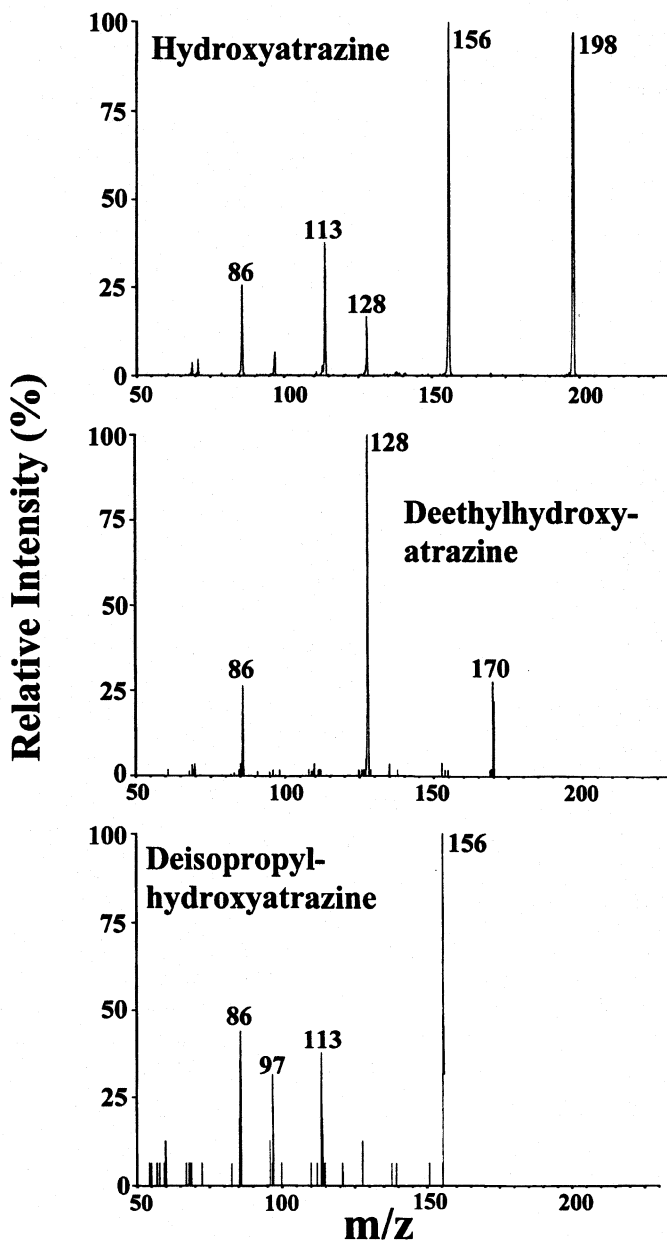
FIGURE 2 LC/MS/MS full scan daughter ion spectra of HADPs isolated from the OH soil. Labeled peaks represent diagnostic daughter ions. Base peak intensities: 326,000 cps for HA; 15,050 cps for DEHA; and 3,200 cps for DIHA
