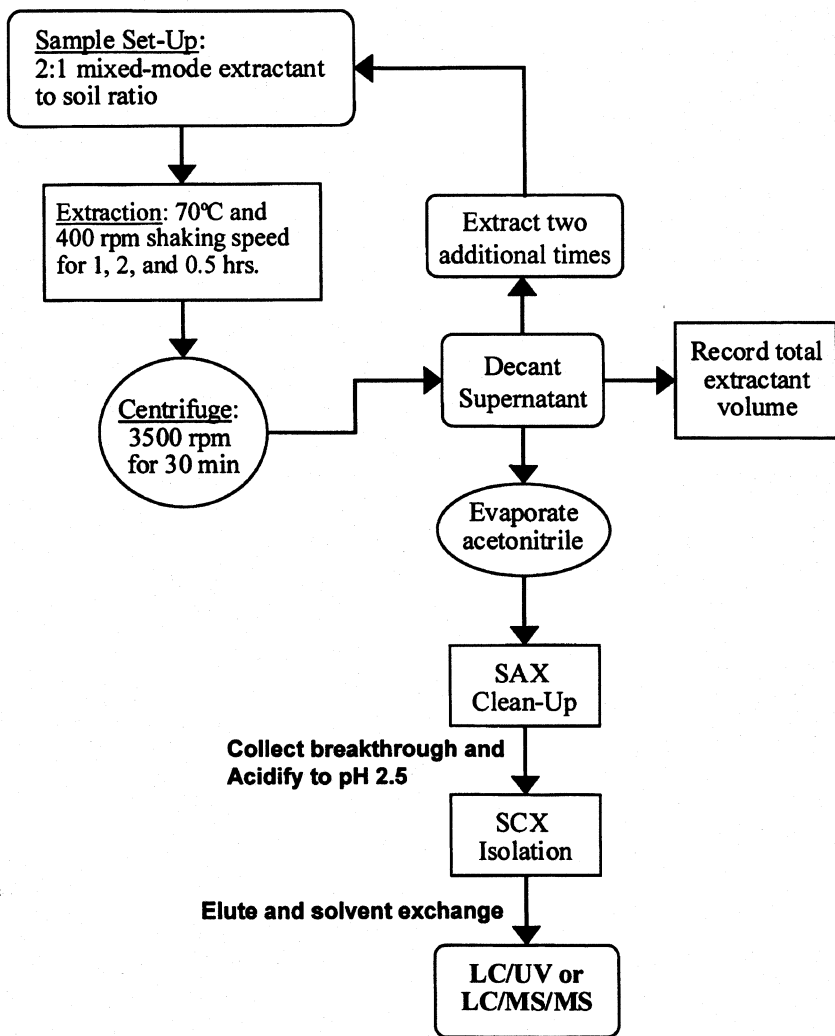
FIGURE 1 Procedural scheme for the mixed-mode extraction of HADPs from soil
