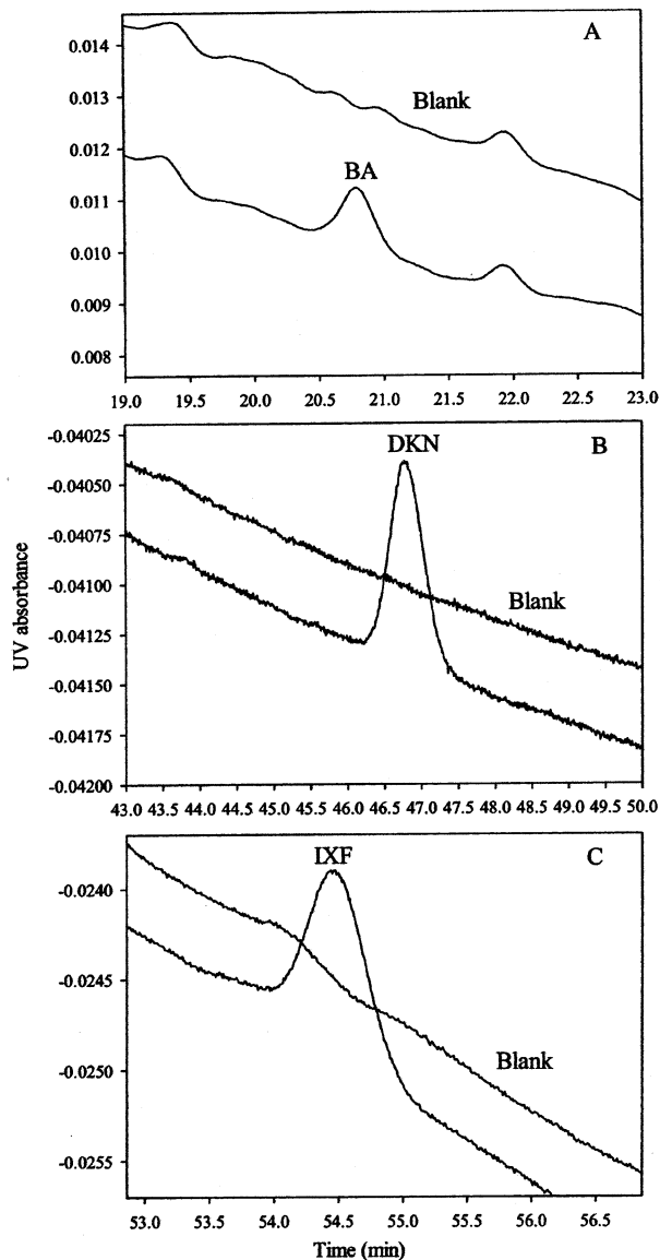
Figure 4. HPLC-UV chromatograms of blank and spiked ground water samples at 1 μg/L using sequential elution of C 18 SPE cartridge: (A) BA; (B) DKN; (C) IXF.
