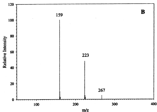
Figure 5. Full-scan mass spectra for IXF and DKN (A) and BA (B). The m/z of the molecular ion is 358 for both IXF and DKN.
