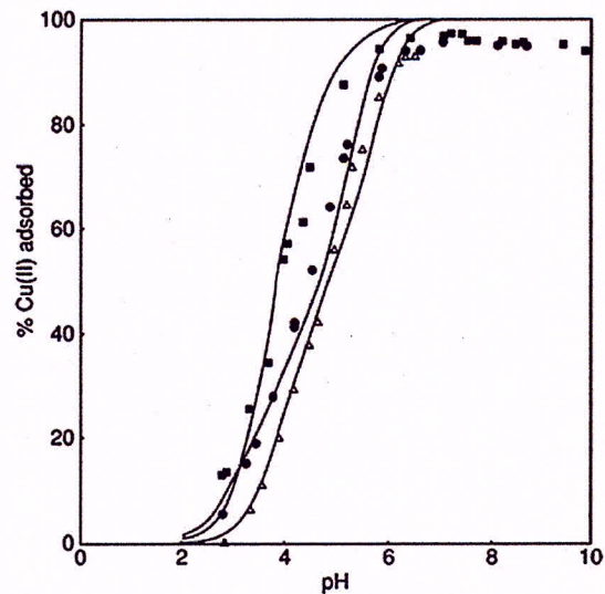
Figure 8 Fit of the diffuse layer model to copper adsorption on lignocellulose extracted from wheat bran. Model fits are represented by solid lines. \Delta [\text{Cu}(\text{II})]_{\text{ini}}=2.10^{-4} \text{ mol l}^{-1} , I=0.1 ; \bullet [\text{Cu}(\text{II})]_{\text{ini}}=2.10^{-4} \text{ mol l}^{-1} , I=0.01 ; \blacksquare [\text{Cu}(\text{II})]_{\text{ini}}=2.10^{-5} \text{ mol l}^{-1} , I=0.1 . Reproduced with permission from Ravat, C., Dumonceau, J., and Monteil-Rivera, F. (2000). Acid/base and Cu(II) binding properties of natural organic matter extracted from wheat bran: modeling by the surface complexation model. Water Research 34, 1327–1329.
