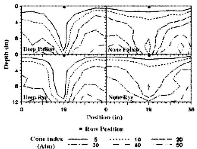
Fig. 2. Contours of cone index as a function of depth into the profile and position across the row averaged over disked and non-disked treatments in 1995. Labels are for deep tillage or none and fallow or rye winter cover.
