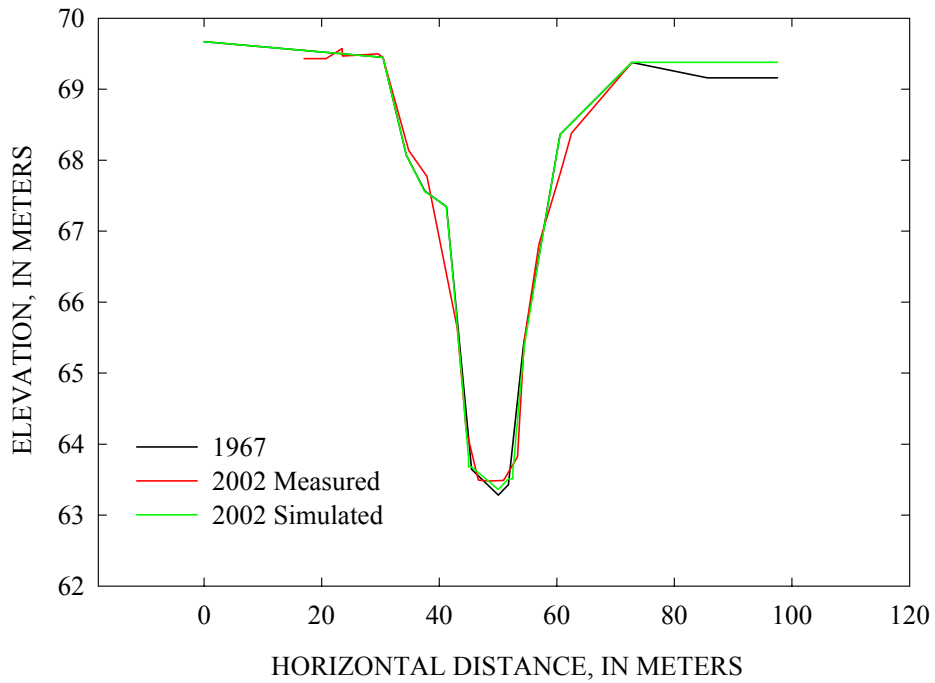
Figure 100 – Comparison of 1967 and 2002 measured with 2002 simulated cross-section 548+70.
