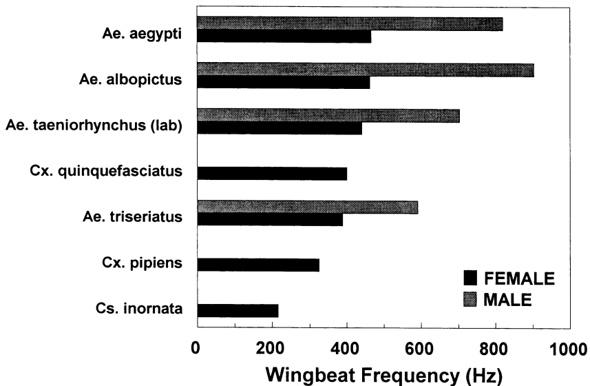
Fig. 5. Comparison of average wingbeat frequencies of different mosquito species. References: Culex pipiens and Culiseta inornata , Belton and Costello (1979); Aedes triseriatus , Moore et al. (1986); Aedes aegypti and Aedes albopictus , Ikeshoji (1981); Culex quinquefasciatus , Ikeshoji et al. (1987).
