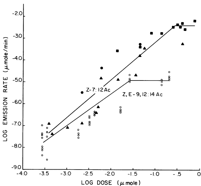
FIG. 1. Release rates of Z-7:12Ac and Z,E-9,12:14Ac from glass dispensers at a flow rate of 50 \text{ cm}^3/\text{min} : Triangles, means of four to seven replications with ^3\text{H} -labeled Z-7:12Ac collected by the air sampler; closed circles, mean of four replications with ^3\text{H} -labeled Z-7:12Ac collected by cold trap; squares, means of 8-19 replications with unlabeled Z-7:12Ac collected by cold trap; open circles, single measurements with ^3\text{H} -labeled Z,E-9,12:14Ac collected by the air sampler.
